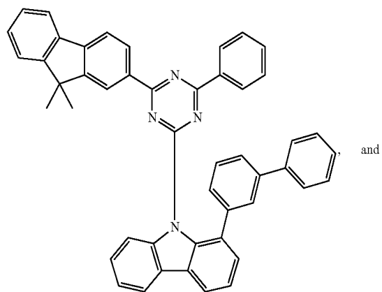
Compound H49
