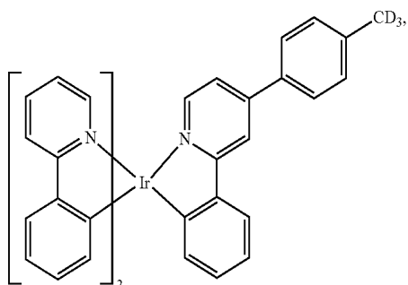
Compound 85
