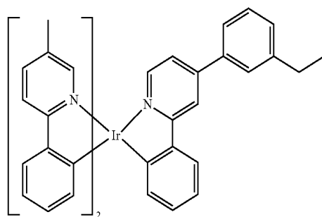
Compound 59
