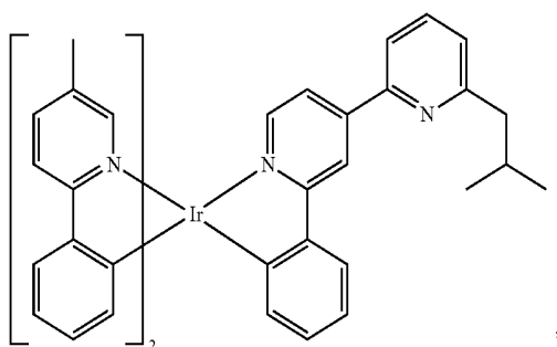
Compound 195
