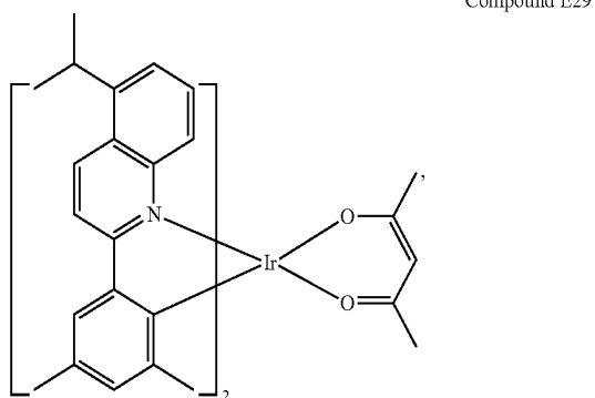
Compound E30
