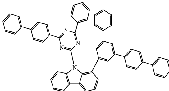
Compound H28
