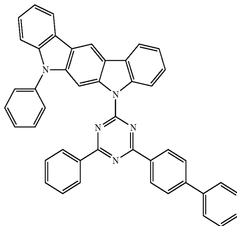
Compound EH19
