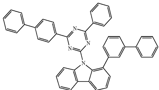
Compound H35
