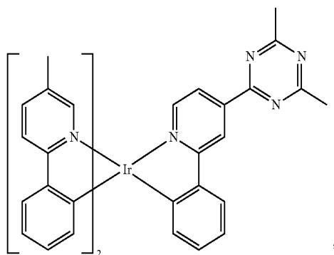
Compound 203
