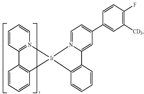
Compound 93
