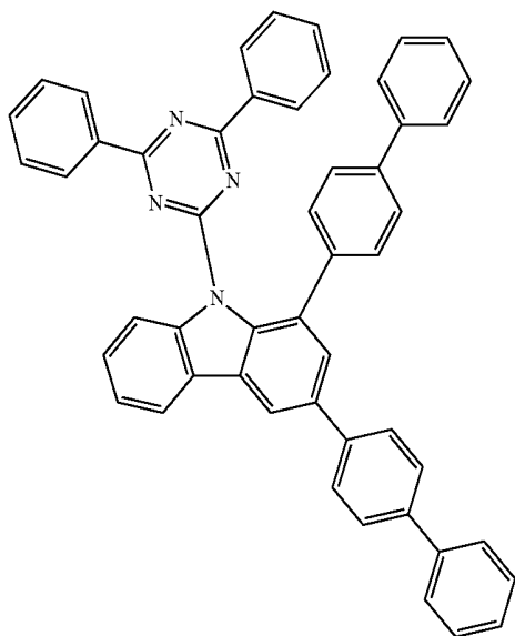
Compound H11
