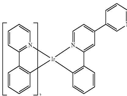
Compound 147
