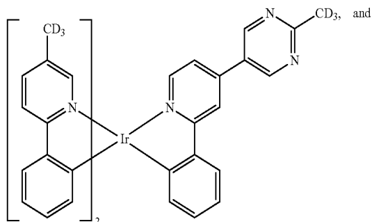
Compound 229
