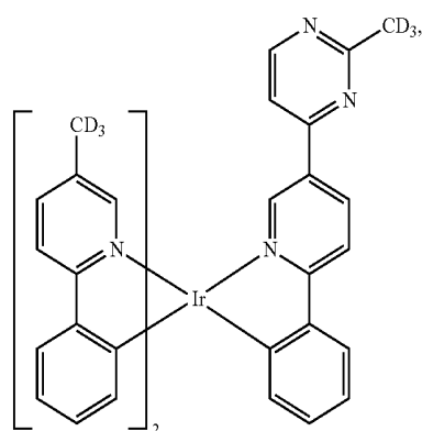
Compound 210
