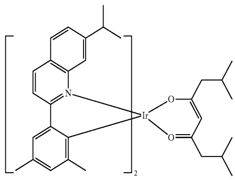
Compound E37
