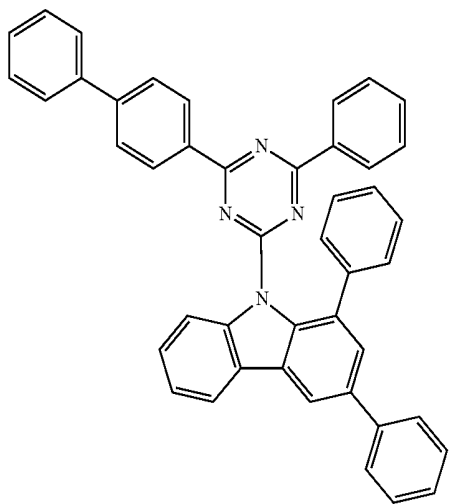
Compound H5
