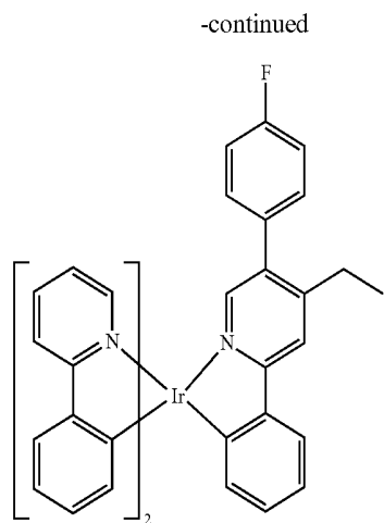
Compound 5
