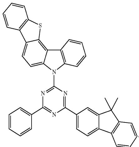
Compound EH36
