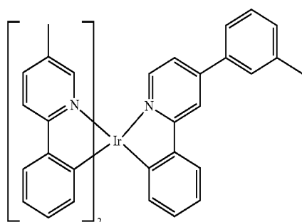
Compound 59
