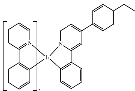
Compound 22
