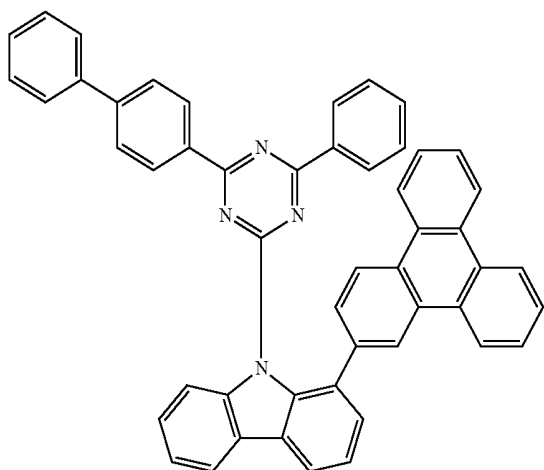
Compound H20
