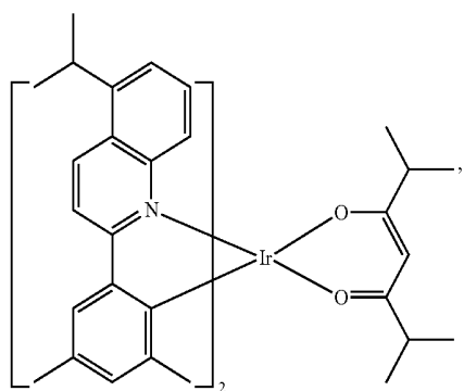
Compound E32
