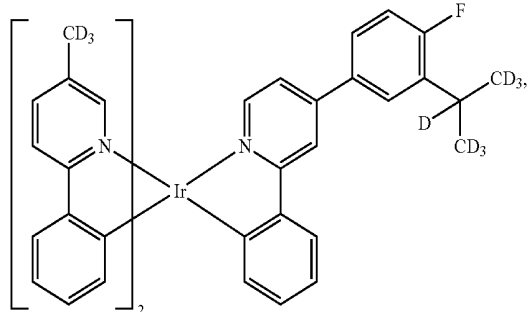
Compound 128
