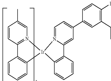
Compound 64
