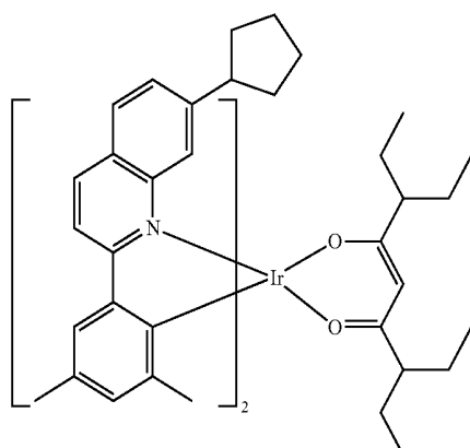
Compound E23
