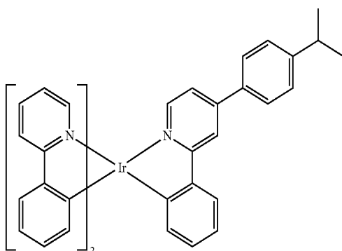
Compound 23
