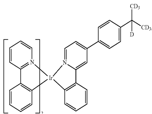
Compound 87
