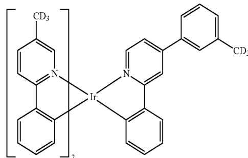
Compound 121
