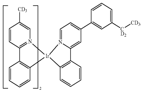
Compound 122
