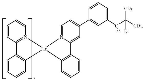
Compound 92
