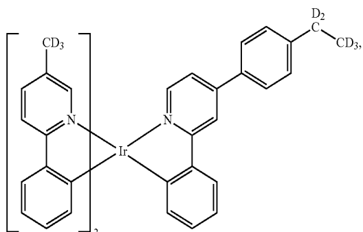
Compound 118
