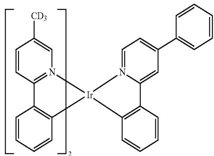
Compound 117
