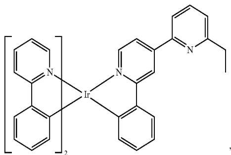
Compound 149
