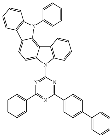
Compound EH33
