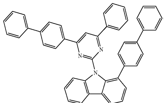
Compound H31
