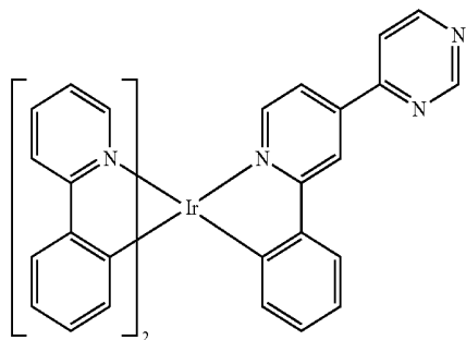
Compound 152
