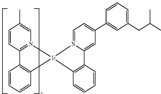
Compound 61
