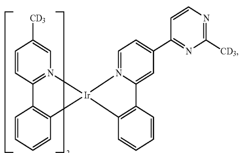
Compound 227
