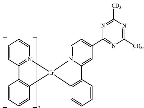
Compound 173
