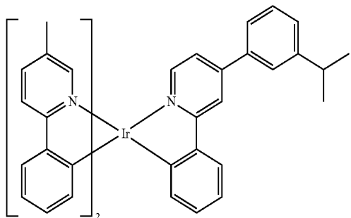
Compound 60
