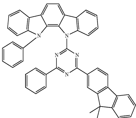
Compound EH5
