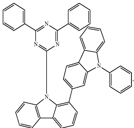
Compound H17
