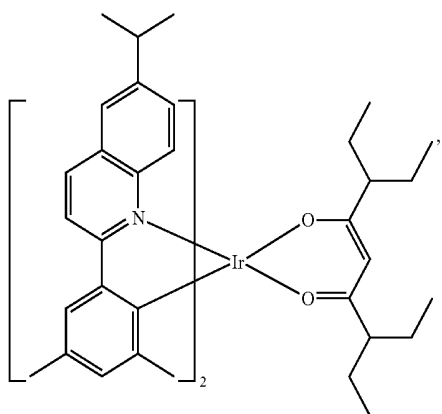
Compound E39
