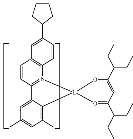
Compound E26
