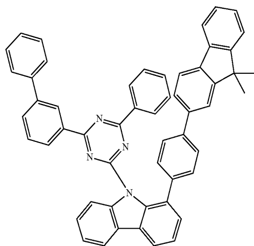
Compound H48
