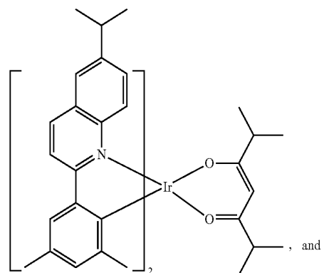
Compound E39
