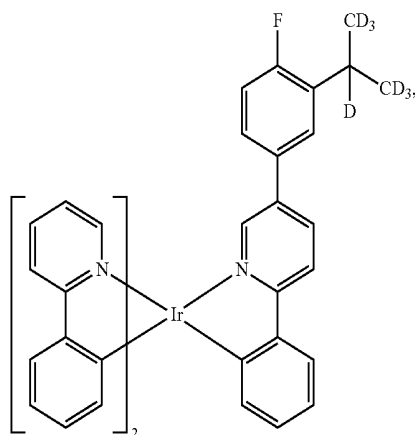
Compound 75
