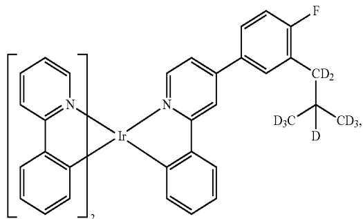
Compound 103
