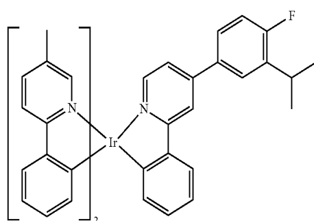
Compound 65
