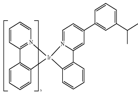
Compound 27
