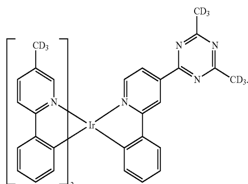
Compound 229
