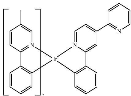
Compound 189
