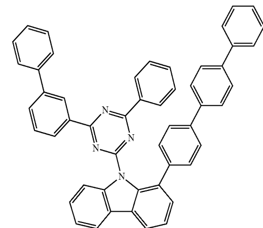
Compound H43
