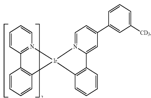
Compound 89
