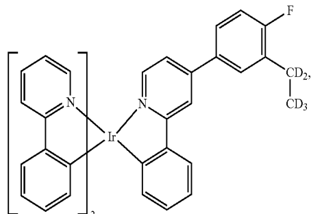
Compound 94
