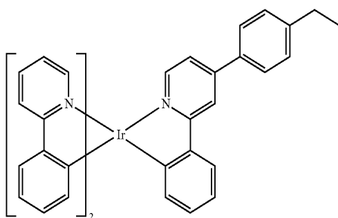
Compound 22
