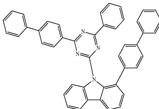
Compound H4
