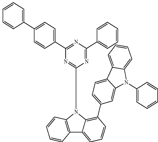
Compound H18
