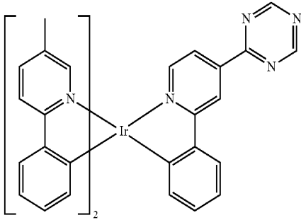
Compound 200
