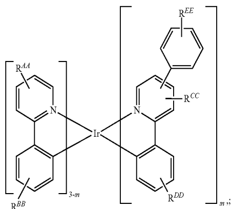
Formula VI
