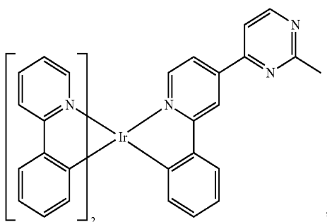
Compound 157
