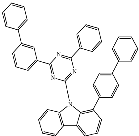
Compound H42
