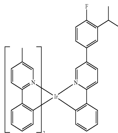
Compound 44
