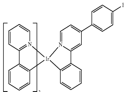
Compound 29
