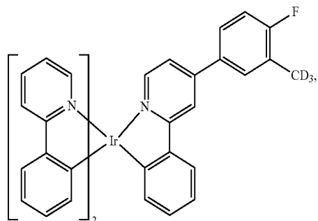
Compound 93
