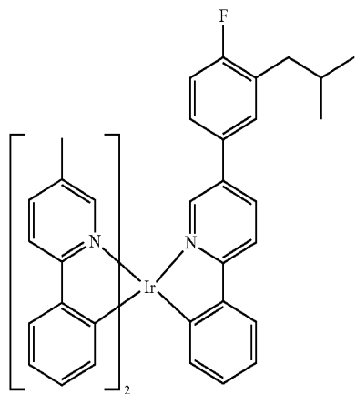
Compound 45
