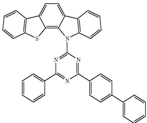
Compound EH4
