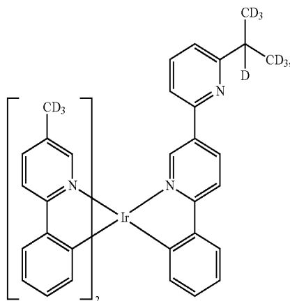
Compound 204
