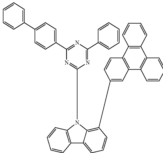
Compound H20
