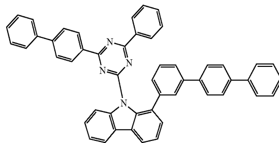
Compound H38
