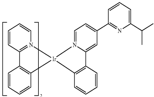
Compound 150
