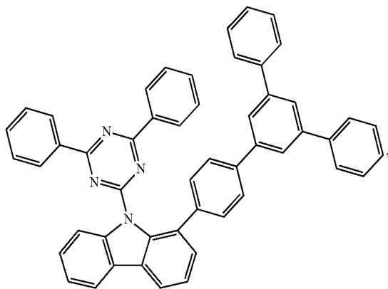
Compound H28
