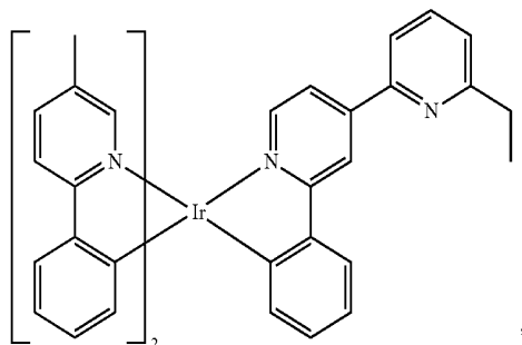
Compound 193
