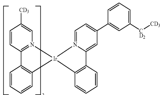
Compound 123
