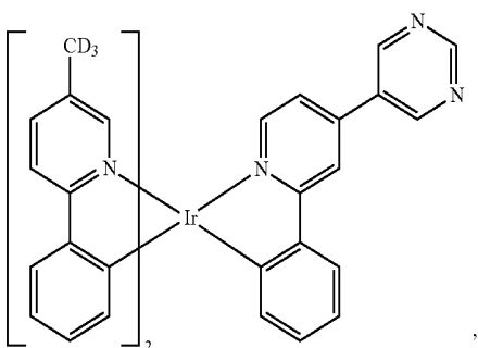
Compound 225
