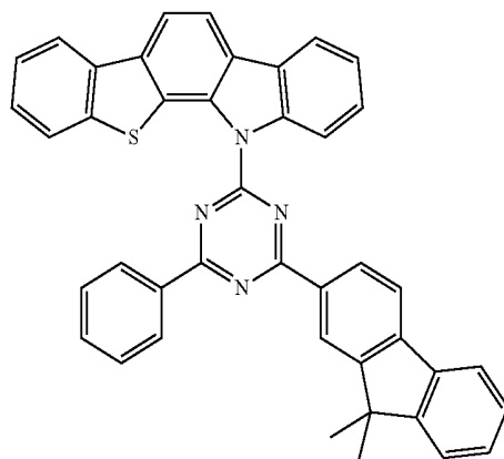
Compound EH7
