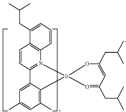
Compound E9
