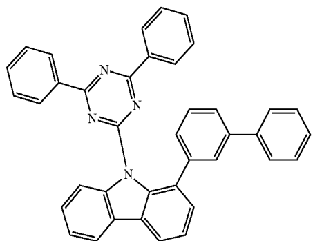
Compound H34
