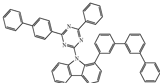
Compound H41
