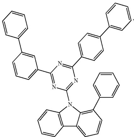
Compound H44
