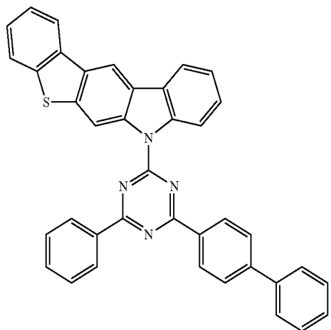
Compound EH22
