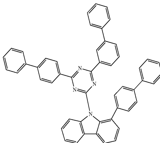
Compound H45
