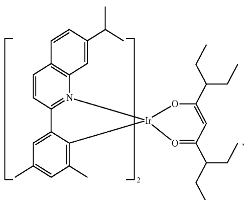
Compound E35
