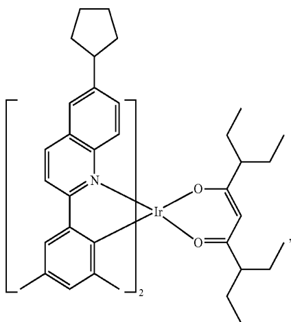
Compound E26
