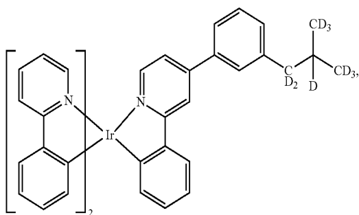
Compound 92
