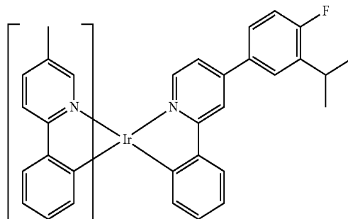
Compound 65
