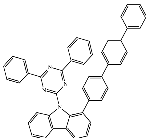
Compound H2
