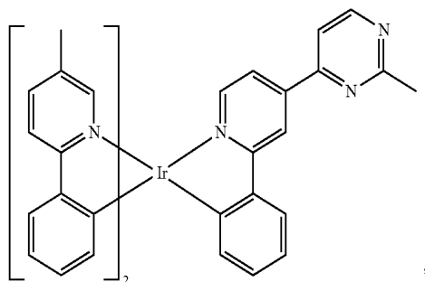
Compound 201
