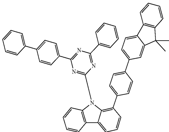
Compound H13
