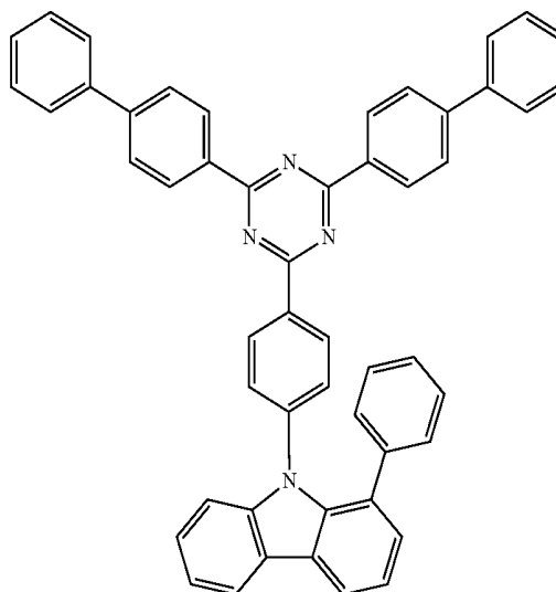
Compound H10
