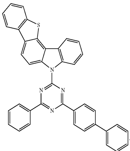
Compound EH35
