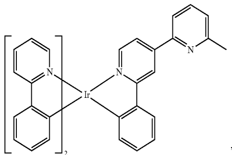
Compound 148
