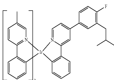
Compound 67
