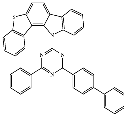
Compound EH45
