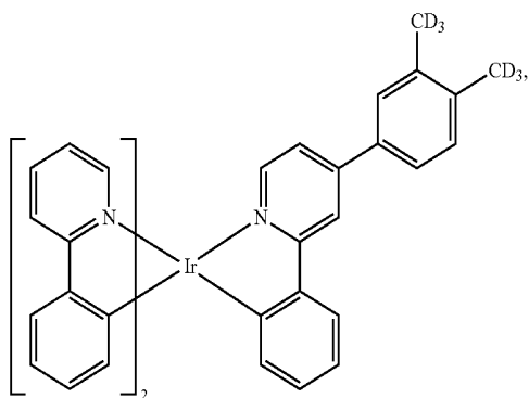
Compound 85
