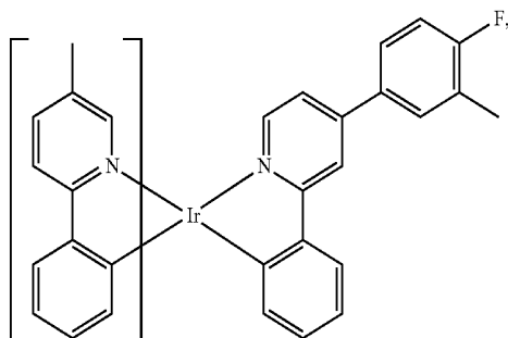
Compound 63
