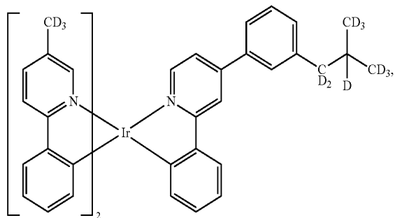
Compound 125
