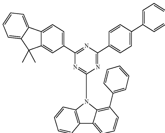
Compound H25
