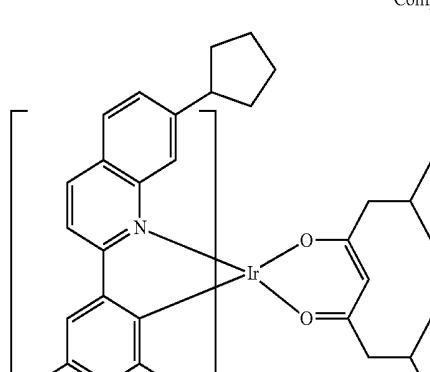
Compound E24
