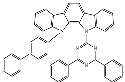
Compound EH1
