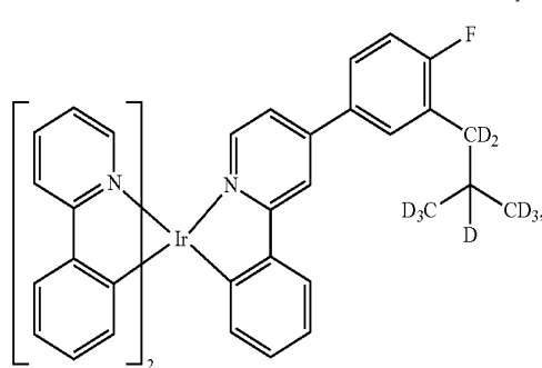
Compound 96
