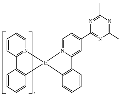
Compound 159
