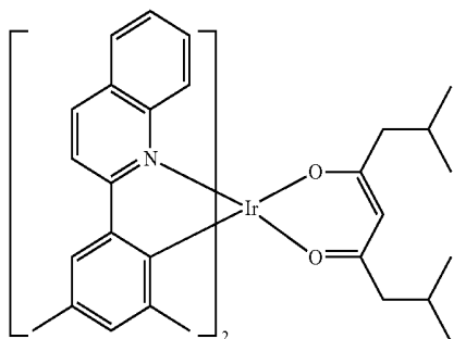
Compound E4
