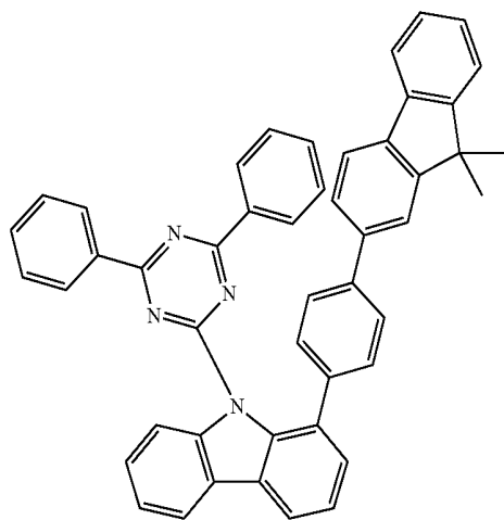
Compound H12
