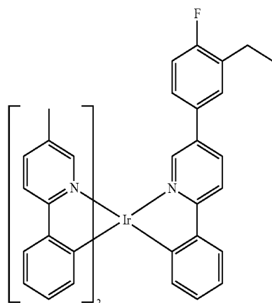
Compound 43
