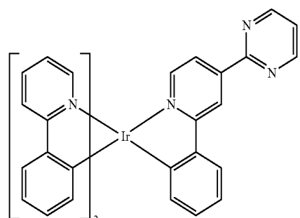
Compound 154
