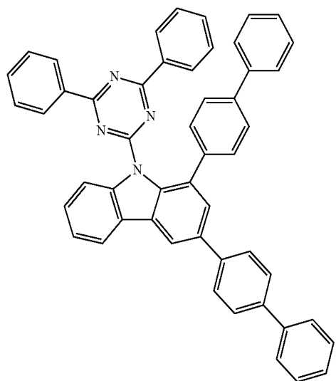
Compound H11
