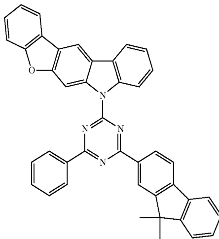
Compound EH26
