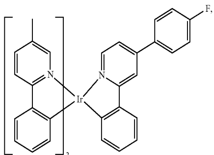
Compound 62
