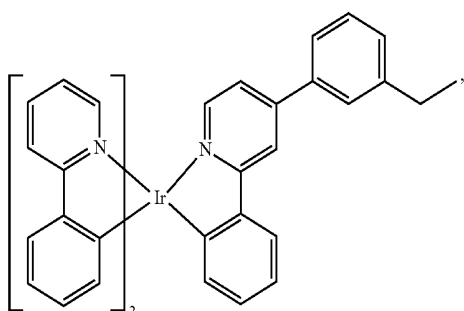
Compound 26
