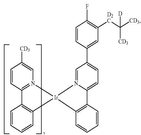
Compound 110
