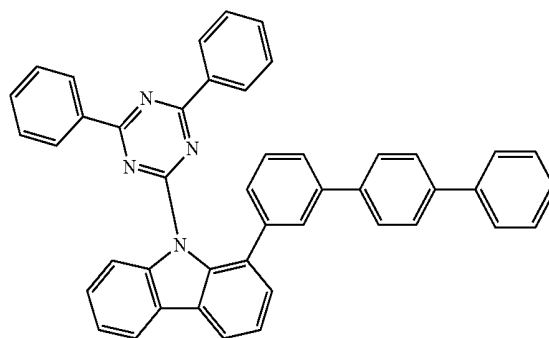
Compound H36
