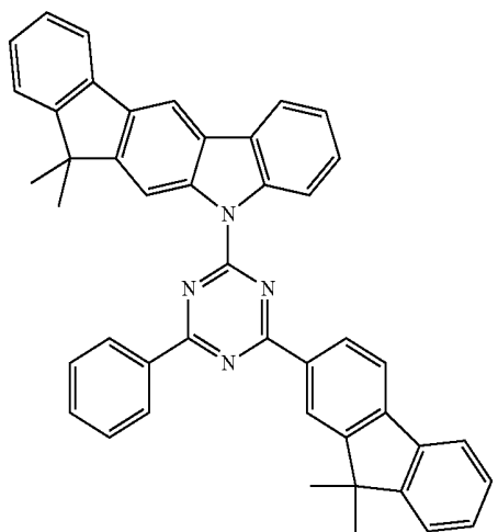
Compound EH29
