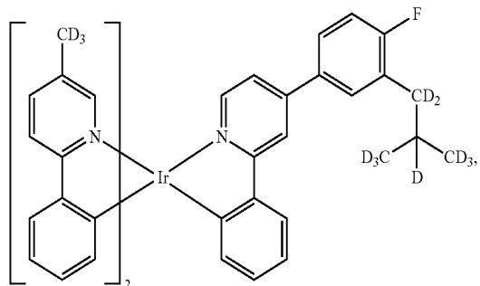
Compound 129
