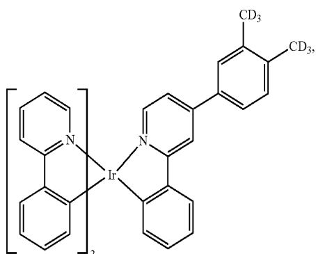
Compound 85
