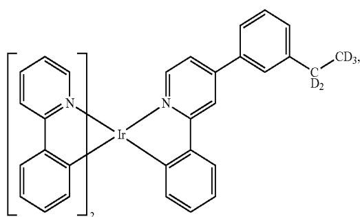
Compound 91
