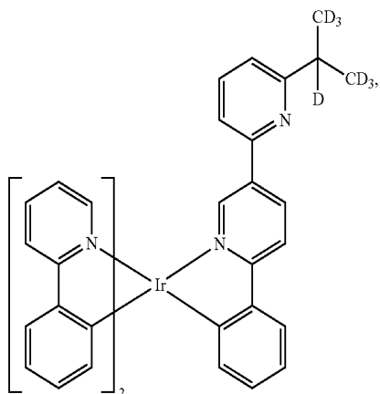
Compound 159
