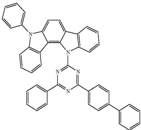
Compound EH42
