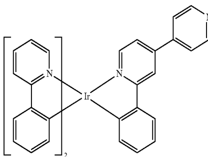
Compound 147
