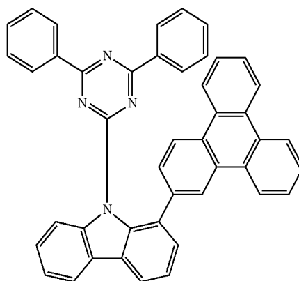
Compound H19
