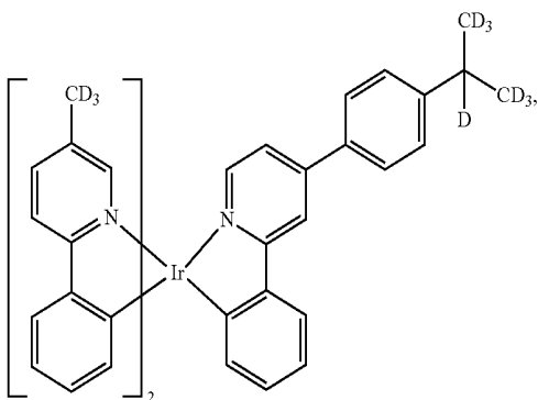
Compound 119
