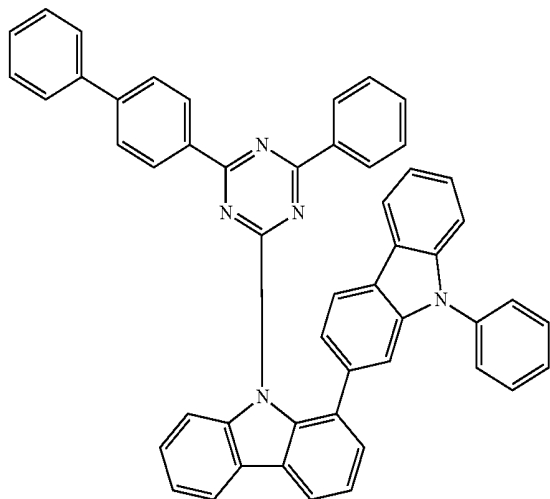
Compound H18
