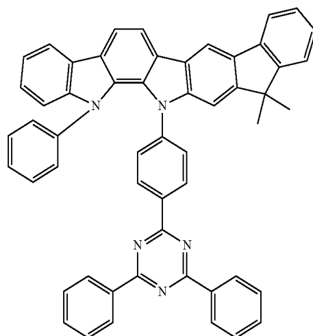
Compound EH53
