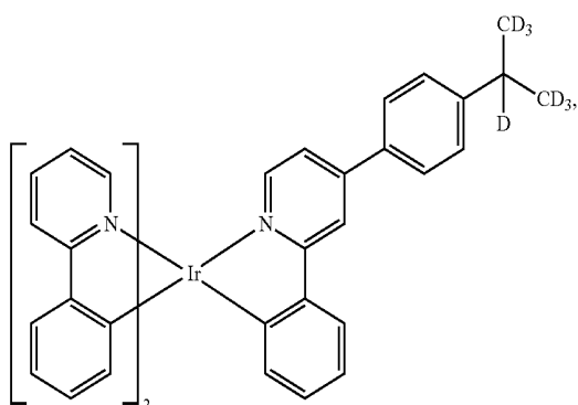
Compound 87
