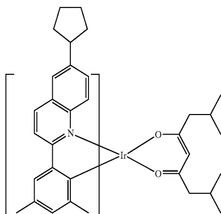
Compound E28
