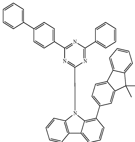
Compound H15
