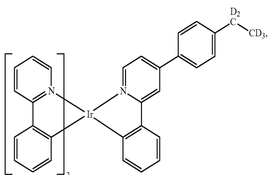
Compound 87
