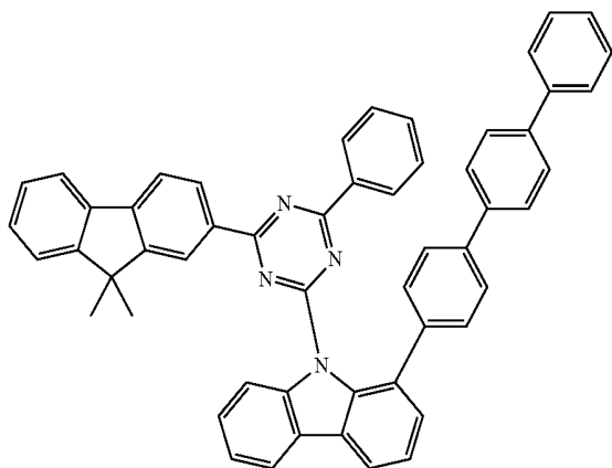
Compound H24
