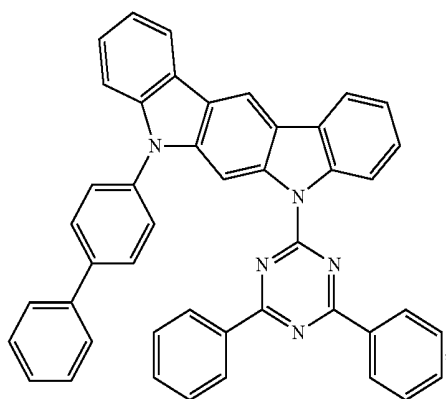
Compound EH18
