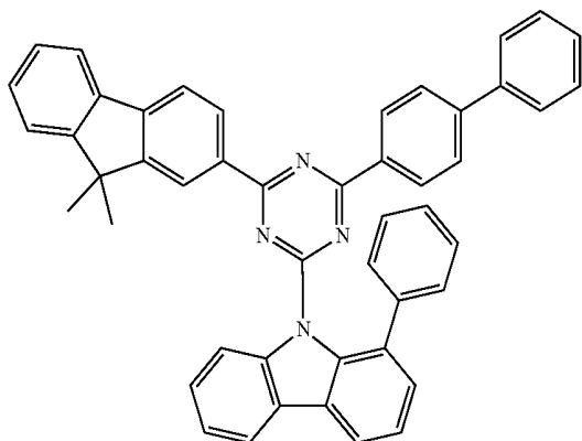
Compound H25
