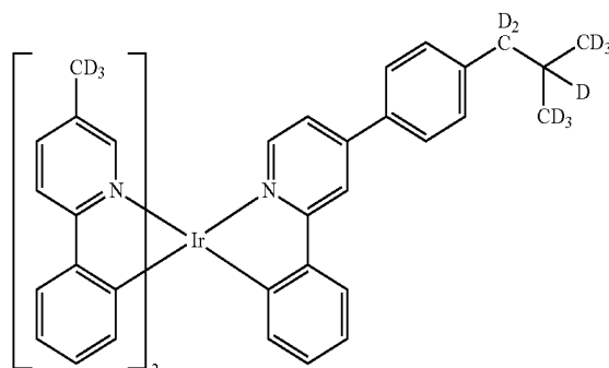
Compound 120
