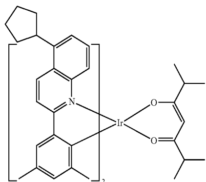
Compound E20
