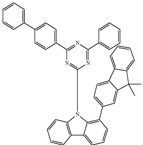
Compound H16
