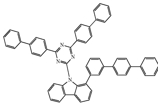
Compound H38
