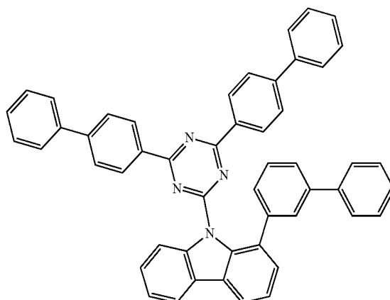
Compound H36
