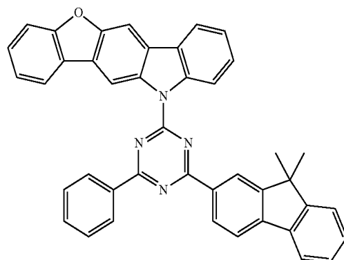
Compound EH15
