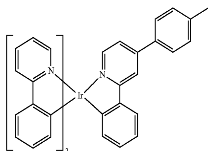
Compound 21
