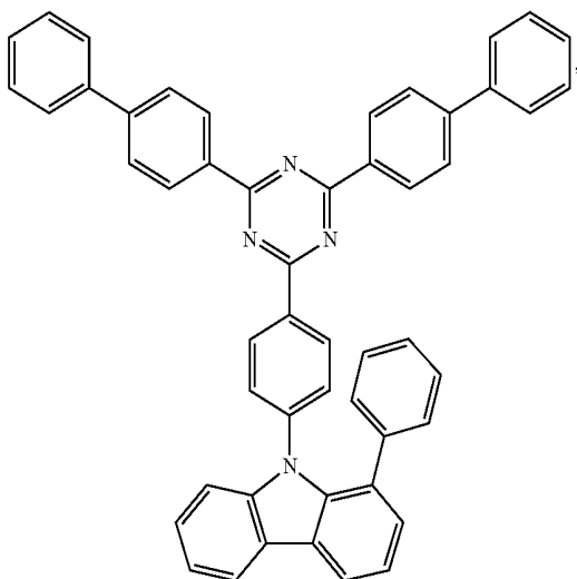
Compound H11
