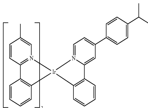
Compound 56
