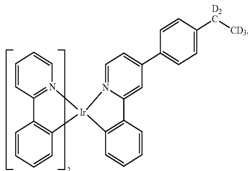
Compound 86
