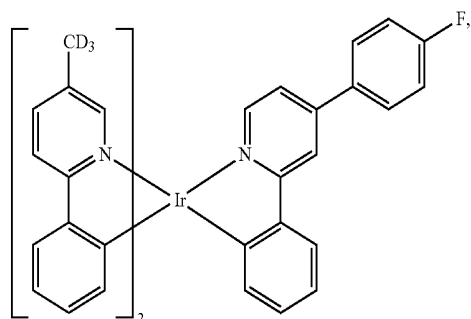
Compound 125
