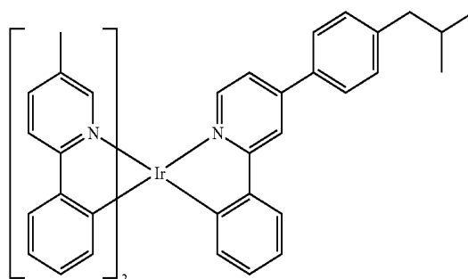
Compound 57
