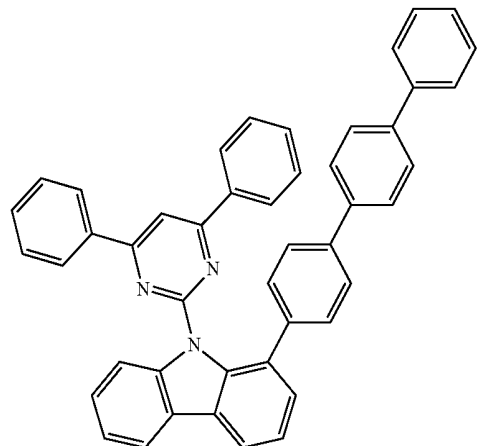
Compound H33
