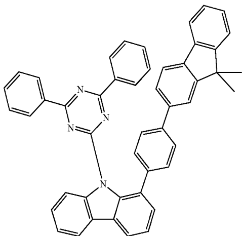
Compound H13
