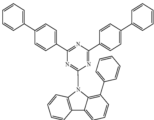
Compound H6
