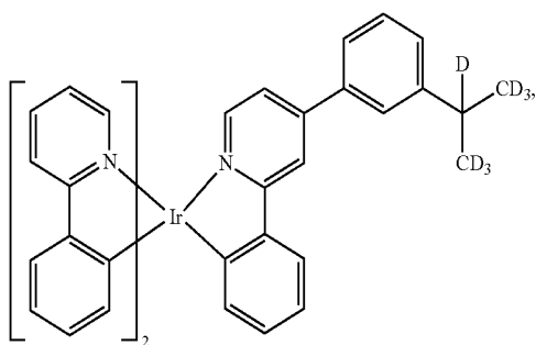
Compound 91
