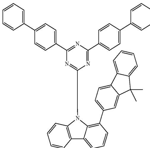
Compound H16
