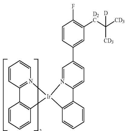
Compound 76
