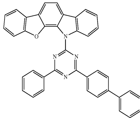
Compound EH6
