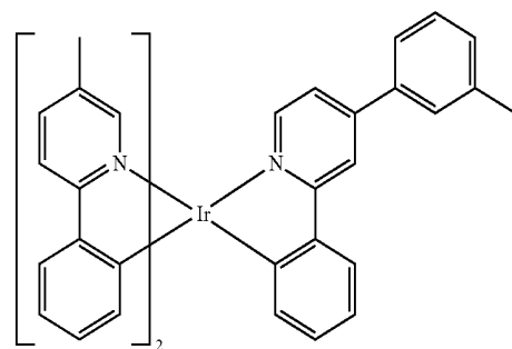
Compound 59
