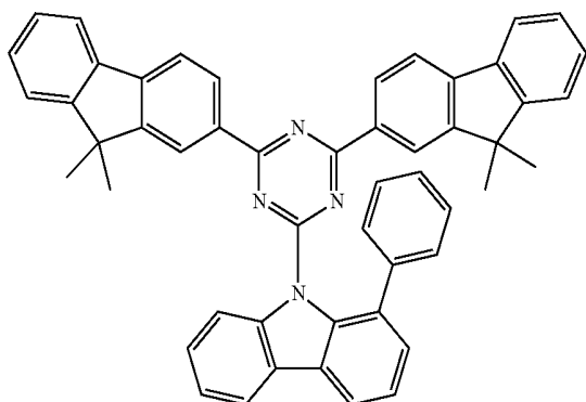
Compound H26
