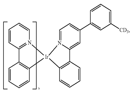
Compound 89
