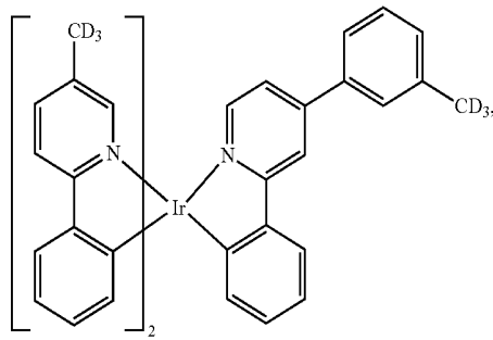
Compound 121
