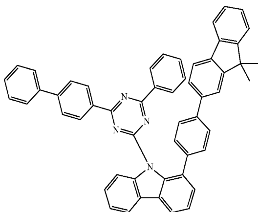
Compound H13
