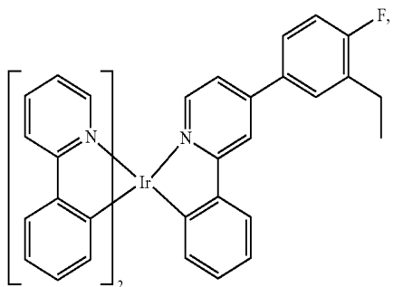
Compound 32
