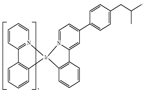
Compound 24
