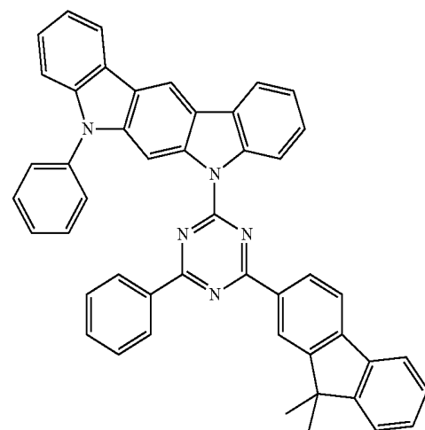
Compound EH20
