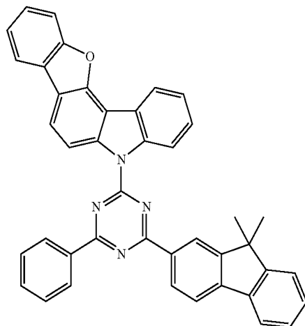
Compound EH39
