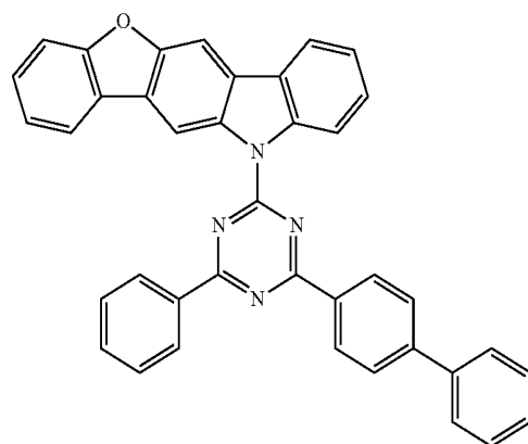
Compound EH14
