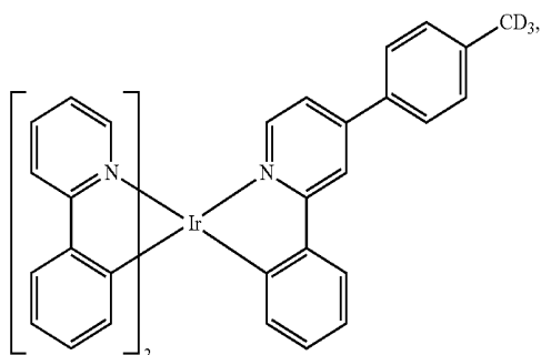
Compound 85
