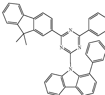
Compound H21
