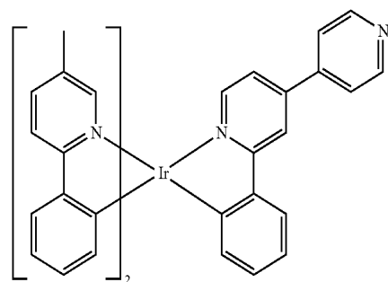
Compound 191
