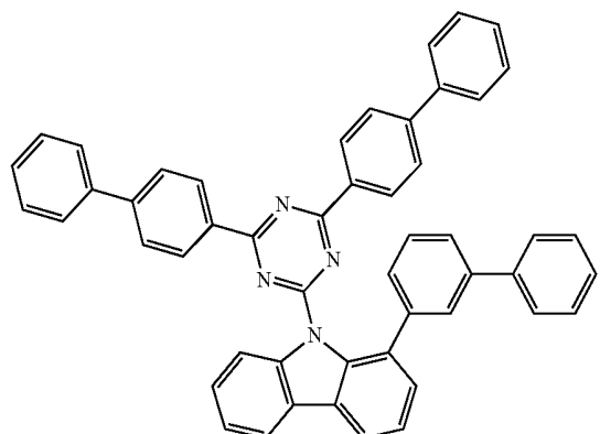
Compound H35
