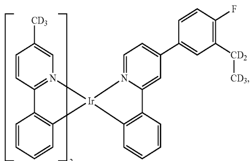
Compound 127
