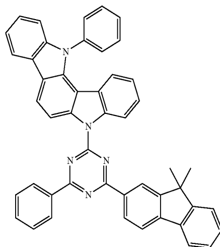
Compound EH33
