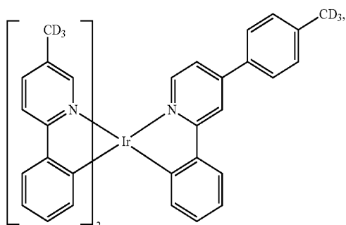
Compound 117
