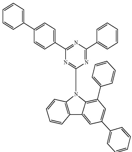
Compound H5
