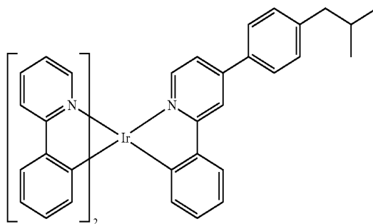
Compound 24
