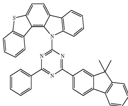
Compound EH45
