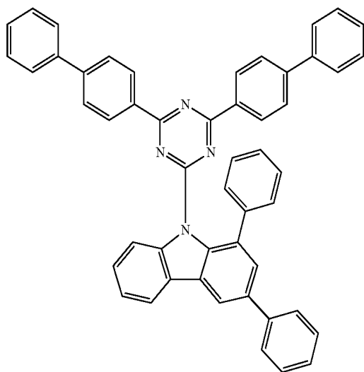
Compound H7
