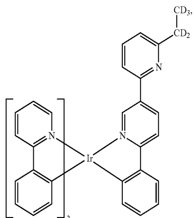
Compound 158
