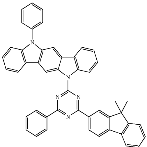
Compound EH16
