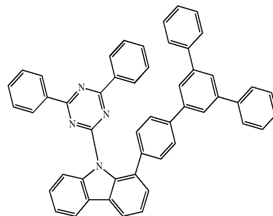
Compound H28
