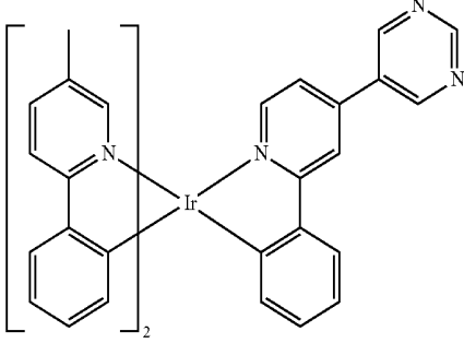
Compound 199
