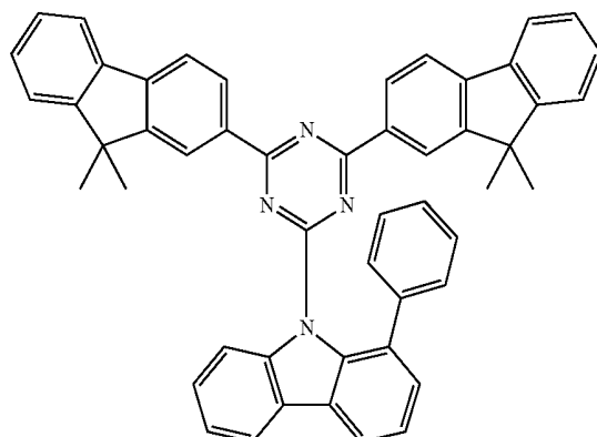
Compound H26
