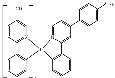
Compound 118
