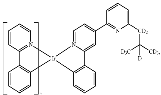
Compound 170
