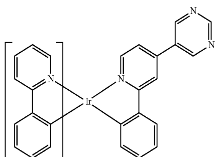
Compound 155
