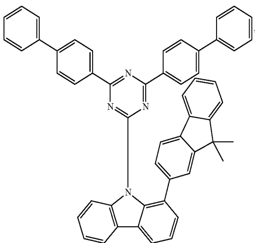
Compound H16
