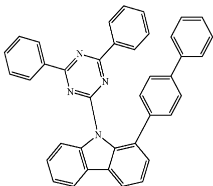
Compound H1
