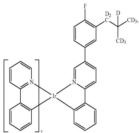
Compound 79
