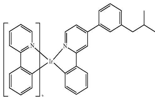
Compound 28
