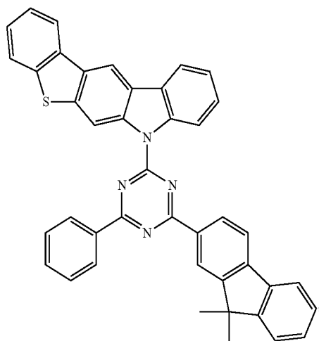
Compound EH23
