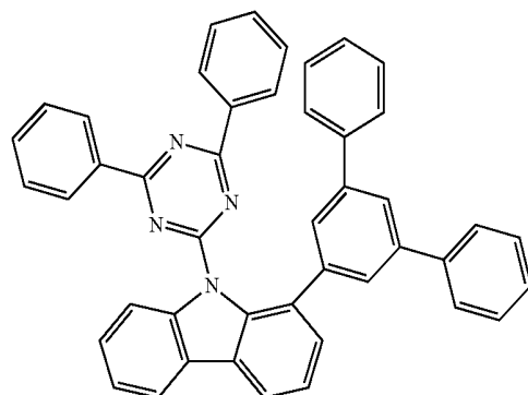
Compound H27
