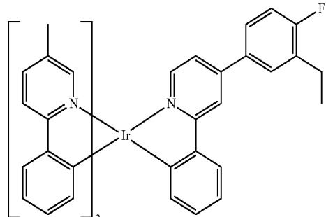
Compound 64
