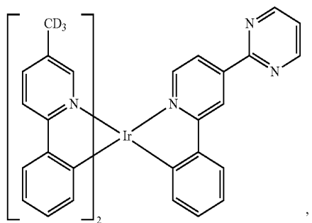
Compound 224
