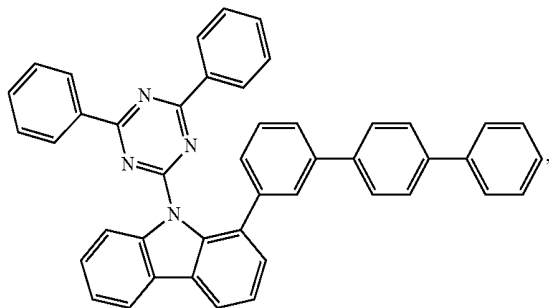
Compound H36
