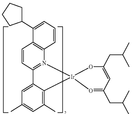
Compound E20
