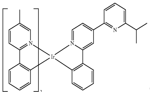
Compound 194
