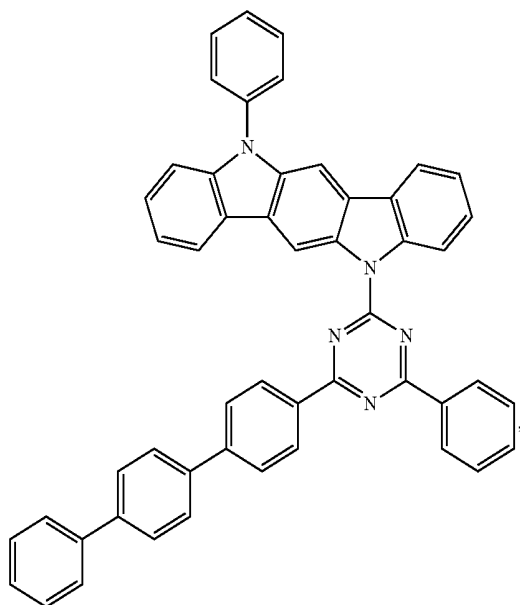
Compound EH9
