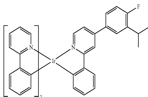
Compound 32
