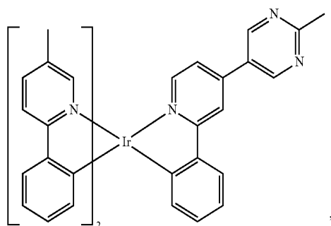
Compound 202
