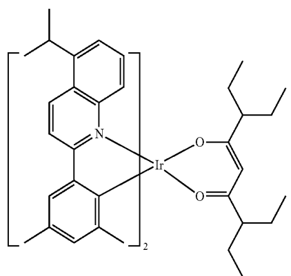
Compound E31
