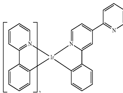
Compound 145
